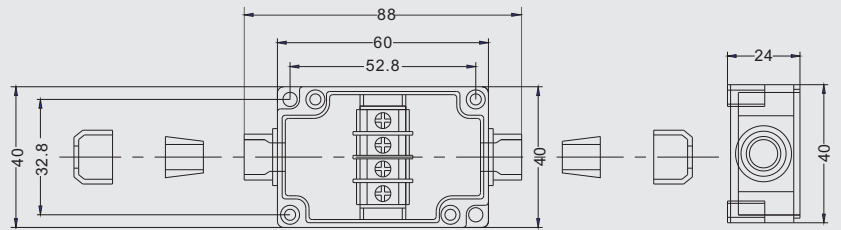
Dimension (允许误差 allowance ±1mm)
