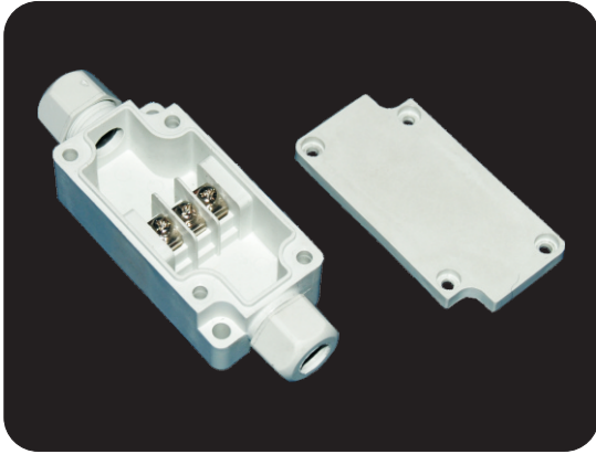
型号 (Model): PBT-3P 尺寸 (Size): 33×65×24mm
