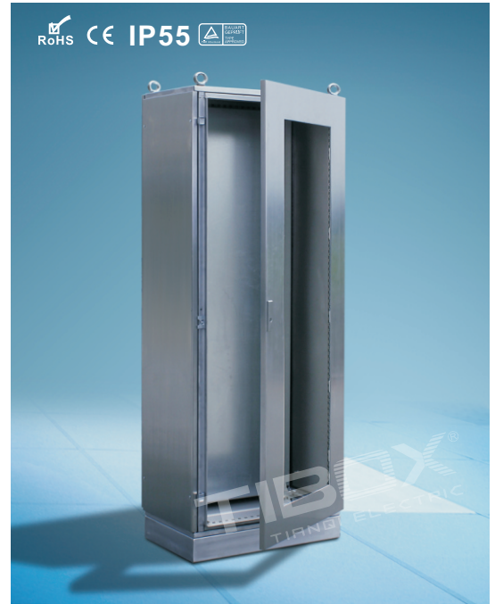
Stainless steel cabinet with glazed door AR9XP type
