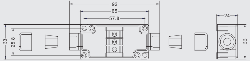
Dimension (允许误差 allowance ±1mm)
