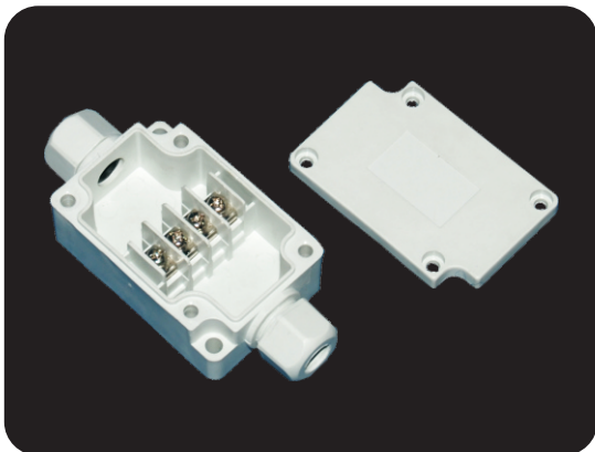
型号 (Model): PBT-4P 尺寸 (Size): 40×60×24mm
