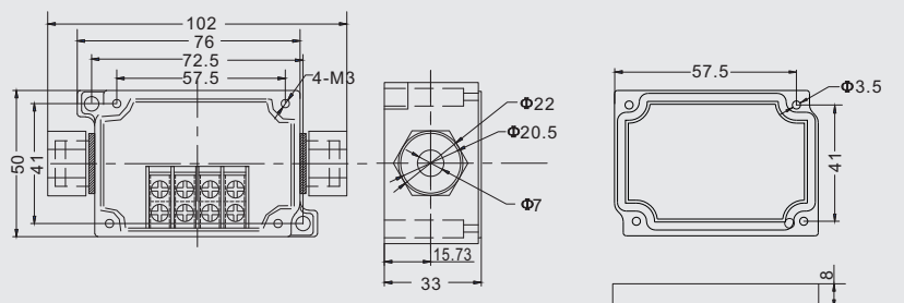
Dimension (允许误差 allowance ±1mm)
