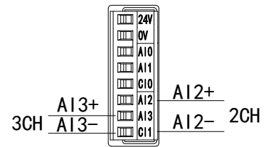
XD-4AD-A-ED current input wiring:
